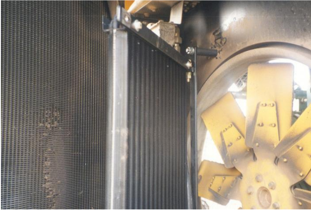
Upper mounting arrangement showing hinge set-up and spacer off shroud.
