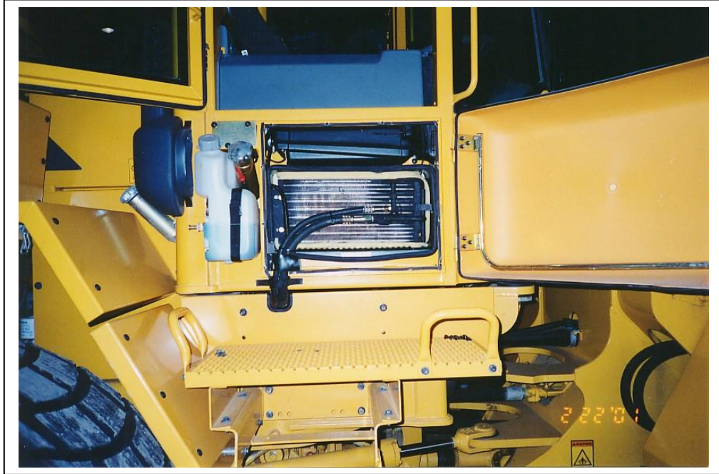
Face on view of evaporator with hoses and thermostat probe.
