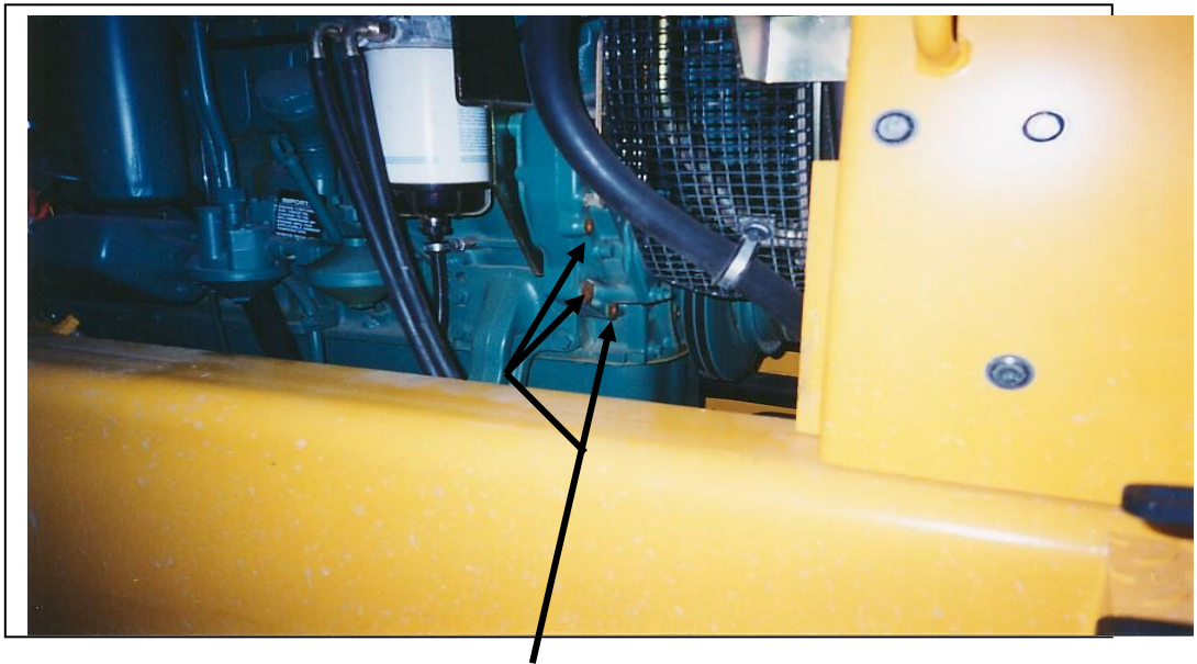
3 holes for compressor mount and stiffener bracket
