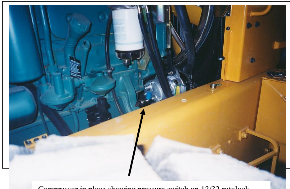
Compressor in place showing pressure switch on 13/32 rotolock
